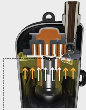
The intermediate pressure keeps pressing the movable scroll during low-load operation.
